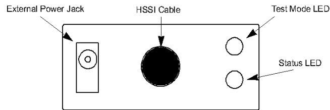
Figure 9. Model 2040 Rear Panel
