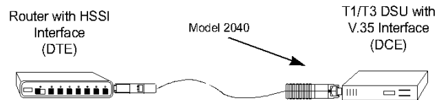
Figure 8. A Common HSSI DTE to V.35/RS-422 DCE Installation
