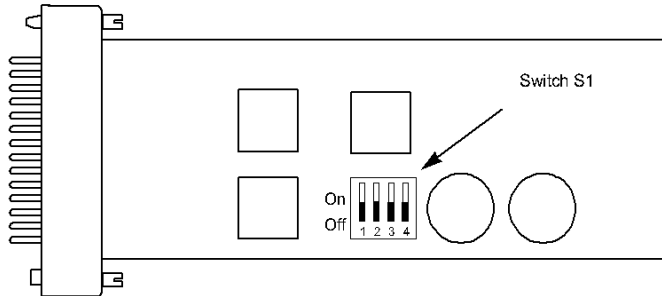
Figure 5. The Model 2040 MT-MC Assembly Drawing
